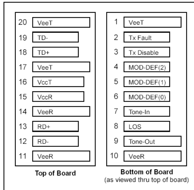
Figure1.Electrical Pin-out Details
