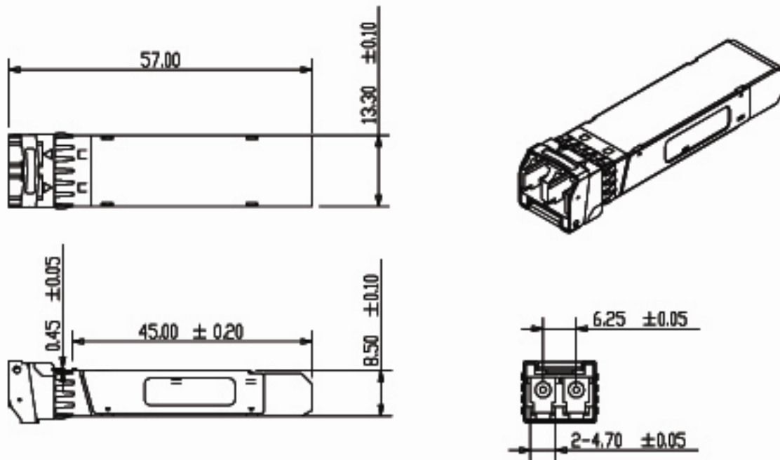
Figure5. Mechanical Dimensions
